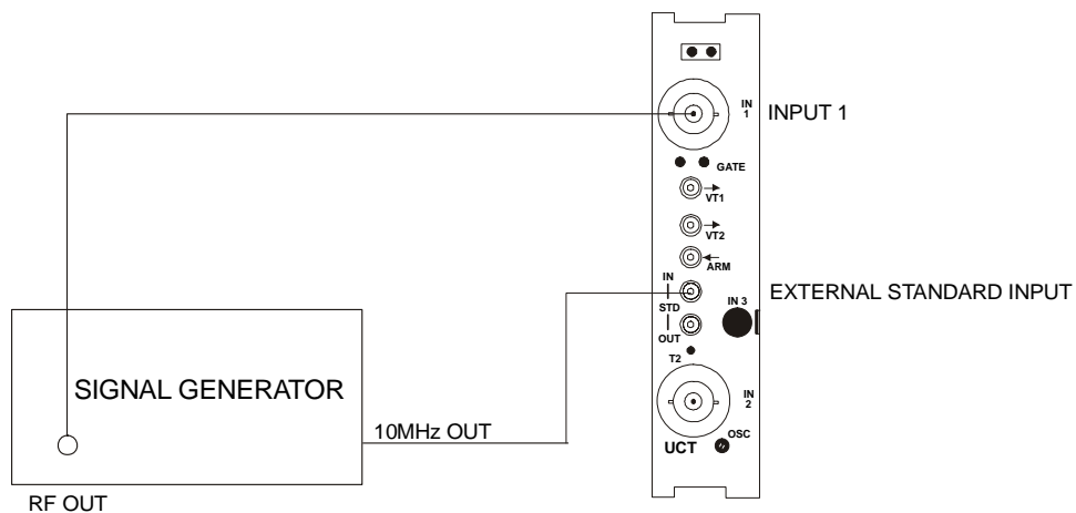
Figure 7-3, Time Interval 1-2 Test Configuration
