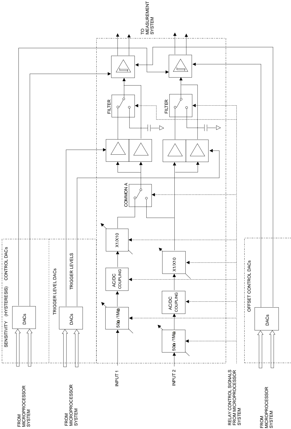
Figure 3-1, Inputs 1 & 2
