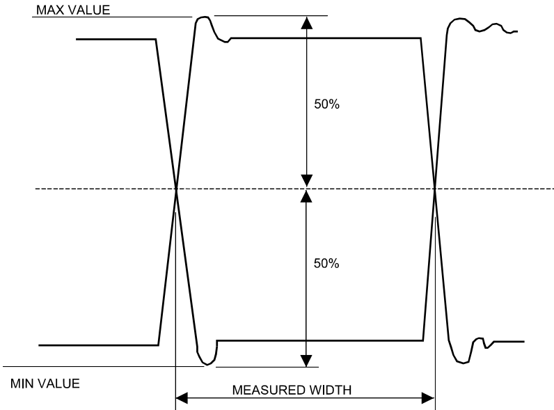
Figure B-1, Positive/Negative Pulse
