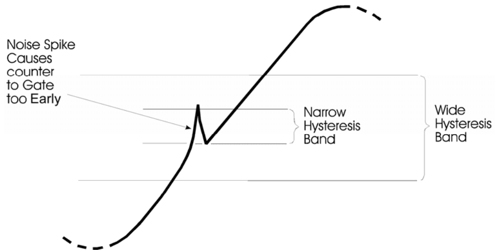
Figure 1-4, Selectable Sensitivity
