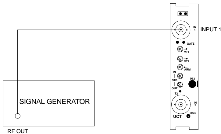
Figure 7-9, Input 1 X10 Attenuator Check Configuration
